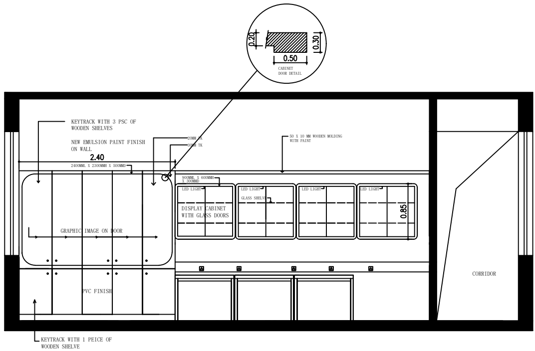
ELEVATION AA
