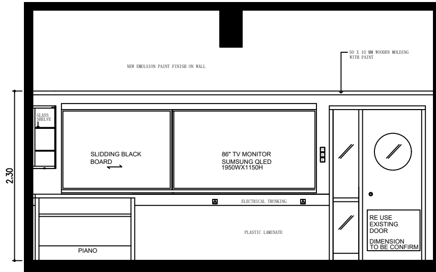
ELEVATION CC
